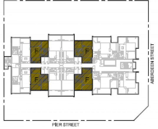
THIRD TO THIRTEENTH FLOOR PLAN
