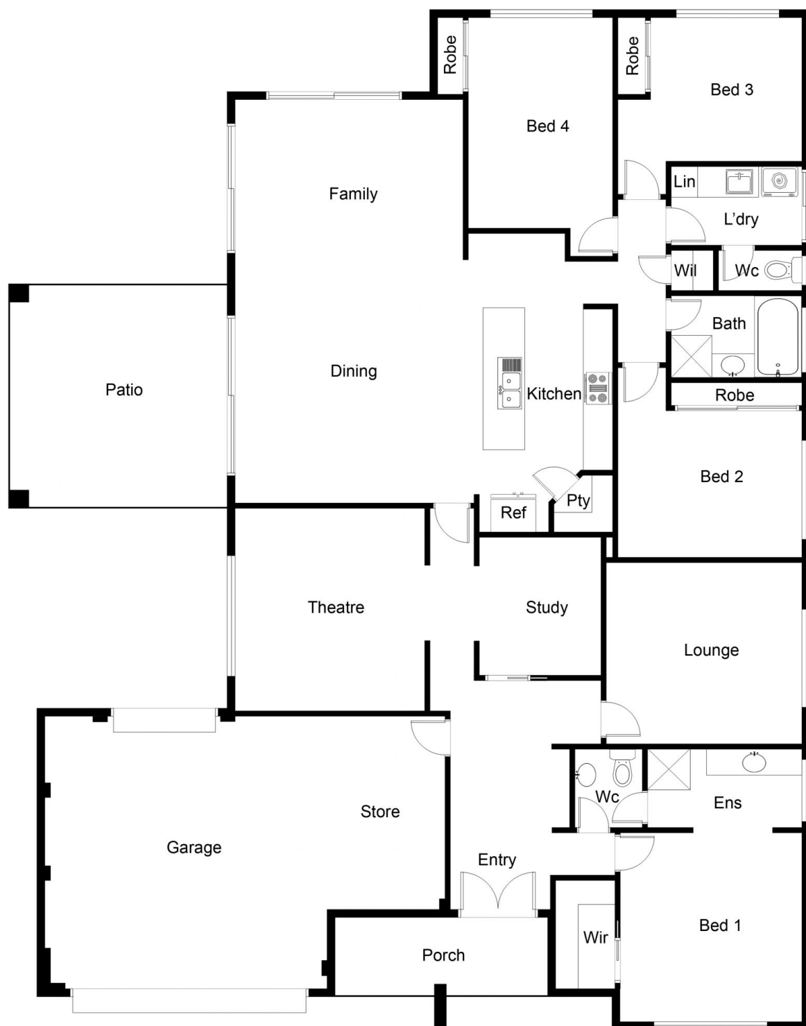
FLOOR PLAN
